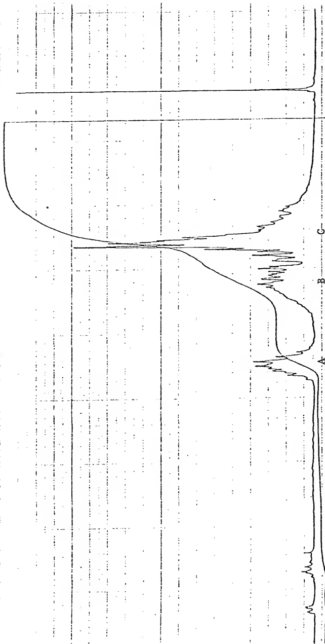
Figure 8 - ^1\text{H} NMR of \text{CF}_3\text{BrCFClCH}_2\text{CHBrCF}_3 \text{C B C A}
